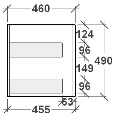
WALL HUNG SIDE VIEW
